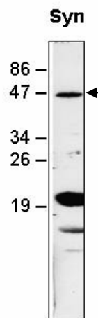
Immunoblot analysis of Synechocystis sp. PCC 6803 membrane proteins with anti-HtrA
